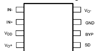
8 Pin MSOP Package
