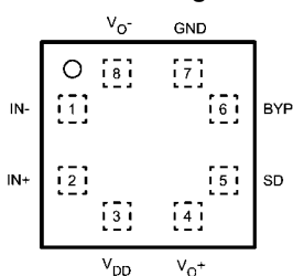
LQ Package
